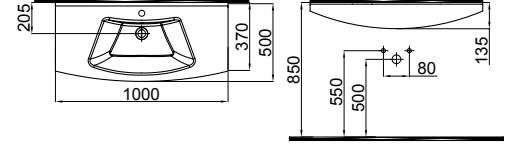
2801-1005 Vega Lavabo / Vega Washbasin (50x100)
