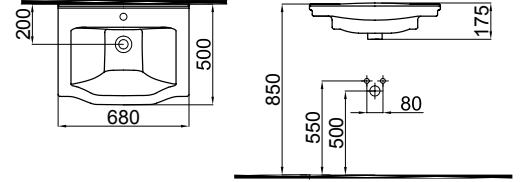
3301-0655 Neo Classic Lavabo / Neo Classic Washbasin (50x65)
