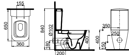
3204-0315 Duvara Sifir Klozet / Back to Wall WC Pan (36x65x40)
