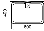
6001-0405 Slim Dikdörtgen (Gizli Sifonlu) Lavabo / Slim Rectangular (Invisible Syphon) Washbasin (40x60)
