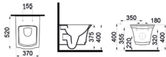
3304-0615 Asma Klozet / Wall Hung WC Pan (37x52x37)
