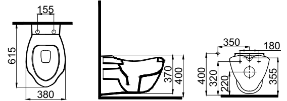
6104-0605 Asma Klozet / Wall Hung WC Pan (38x61x37)
