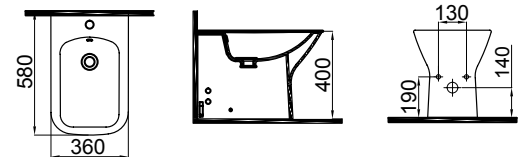
3506-0105 Duvara Sifir Bide / Back to Wall Bidet (36x58x40)
