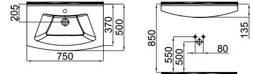
2801-0755 Vega Lavabo / Vega Washbasin (50x75)
