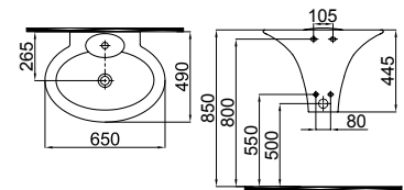
2901-2505 Rena Monoblok Lavabo / Rena Monoblock Washbasin (49x65)
