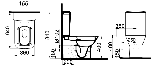
3504-0315 Duvara Sifir Klozet / Back to Wall WC Pan (36x64x40)
