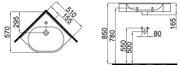
0201-0505 Myra Köşe Lavabo / Myra Washbasin (51x51)
