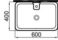
6001-1405 Slim Dikdörtgen Lavabo / Slim Rectangular Washbasin (40x60)
